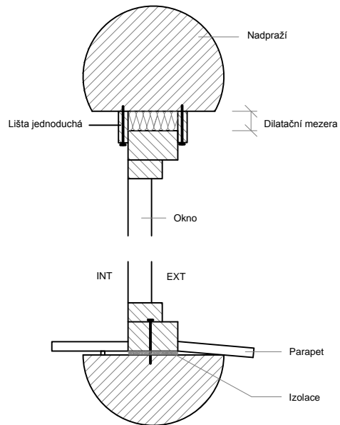
Varianta A (pouze srub)
