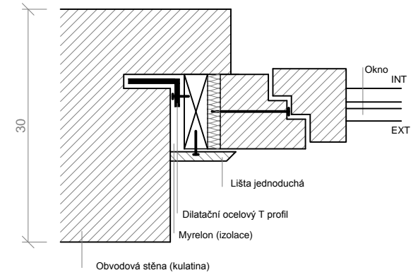
Varianta C (pouze srub)
