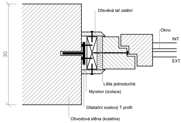
Varianta A (pouze srub)
