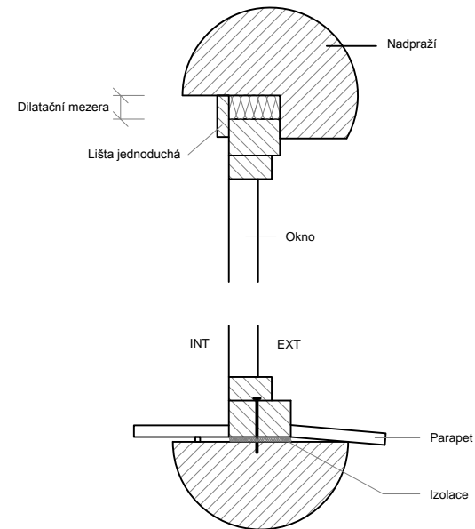
Varianta C (pouze srub)
